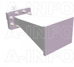
LB-187-10-C-NFSPO Standard Gain Horn Antenna 3.95-5.85GHz 10dB Gain N Type Female
