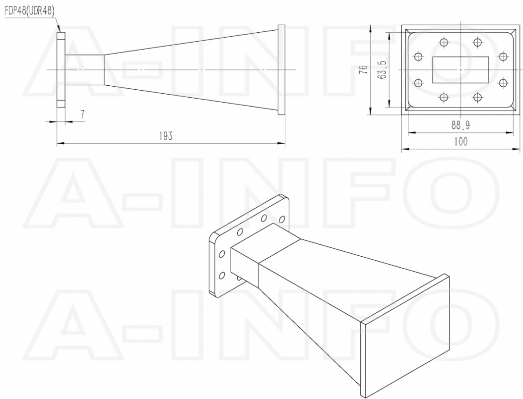
FDP48 Output with Radome (Option, P/N: LB-187-10-ASPO, Outdoor Application)
